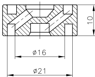
24-R-321 w.st.nr: 1.4541
