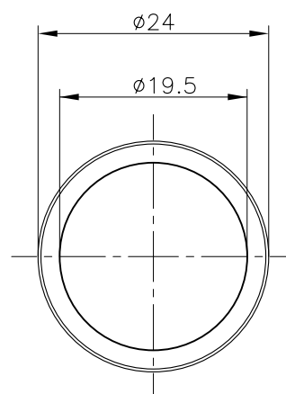
Ring 24 w.st.nr: 1.4122
