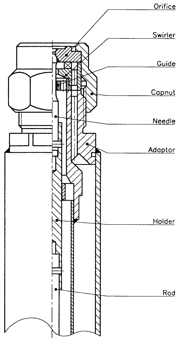
Needle closed
