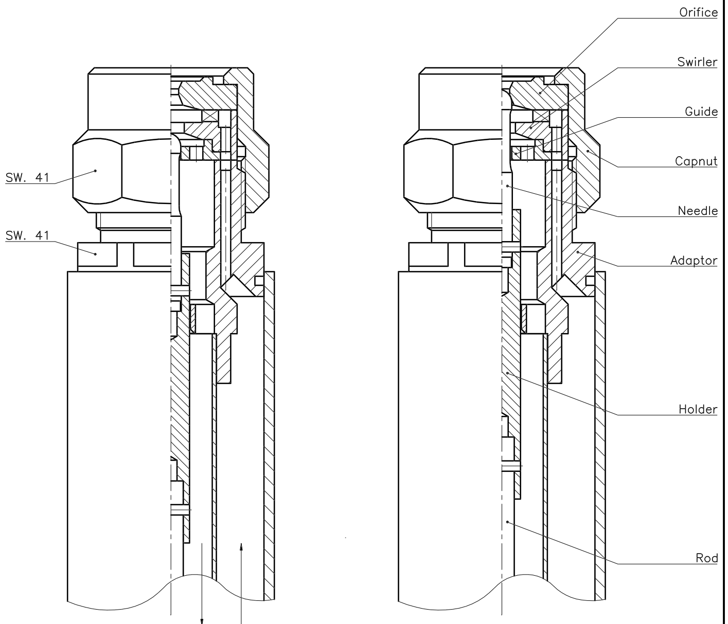
Needle open
