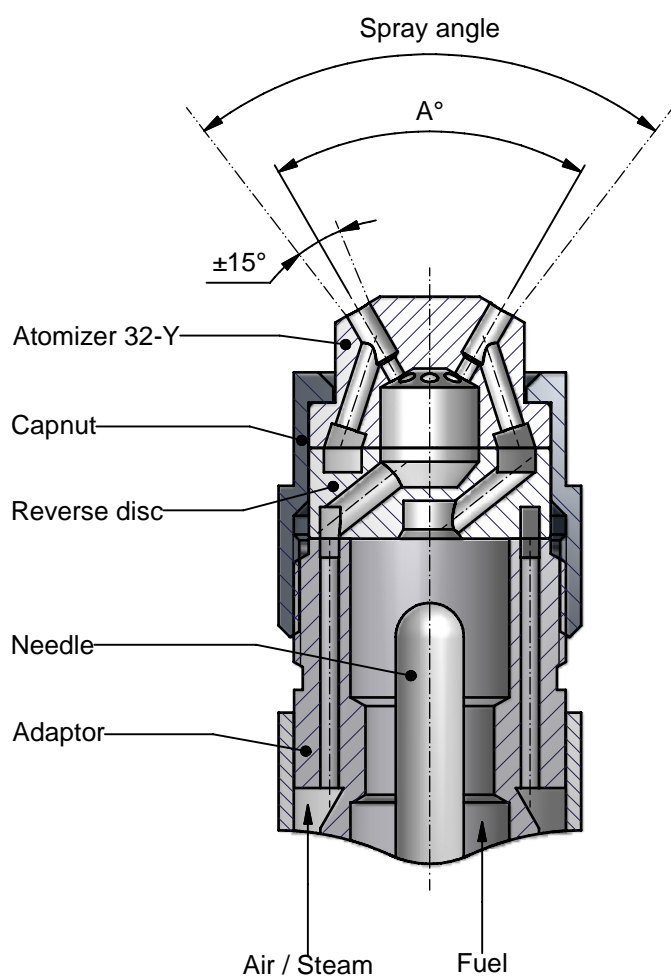
Needle open
