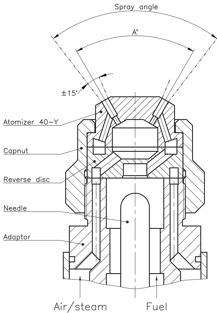
Needle open
